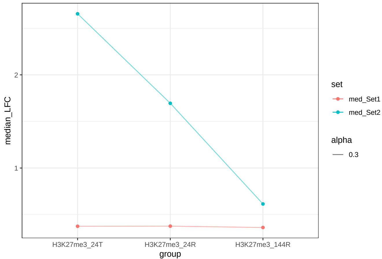
LFC across time for H3K27me3 sets
